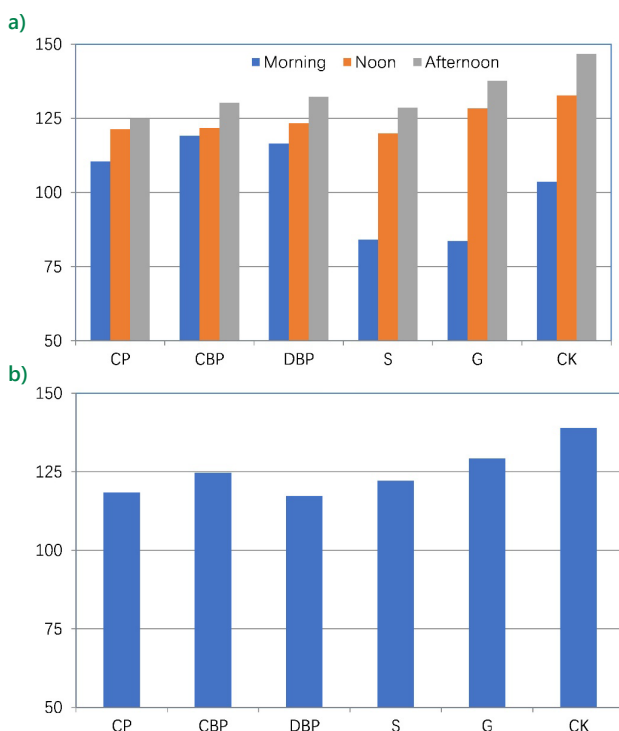
Figure 6. O_3 instantaneous values ( \mu\text{g}\cdot\text{m}^{-3} ) and AQI in different plant community type areas
