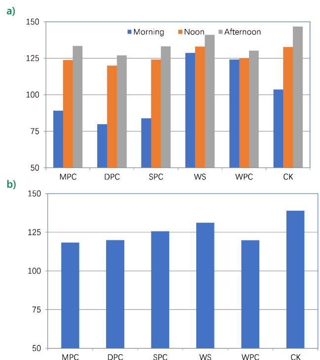
Figure 7. O_3 instantaneous values ( \mu\text{g}\cdot\text{m}^{-3} ) and AQI in typical landscape environment areas
