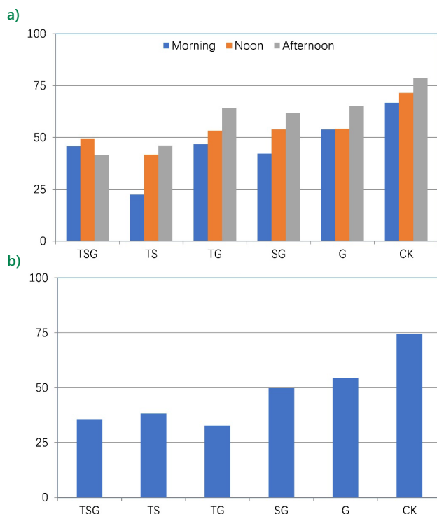
Figure 2. PM_{2.5} instantaneous values ( \mu\text{g}\cdot\text{m}^{-3} ) and AQI in different plant community structure areas
