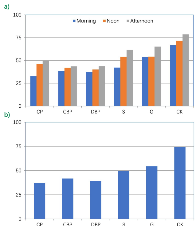
Figure 3. PM_{2.5} instantaneous values ( \mu\text{g}\cdot\text{m}^{-3} ) and AQI in different plant community type areas
